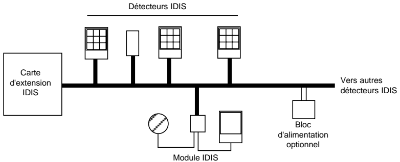
Figure 24. Configuration bus
